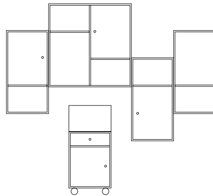
Shelving D 30 cm W 175.8 cm H 115.2 cm RUNNER D 38 cm W 35.4 cm H 66.8 cm Castors H 6.8 cm
