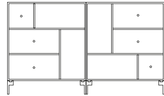
Dresser on legs W 139.2 cm H 69.6 cm Legs H 12.6 cm
