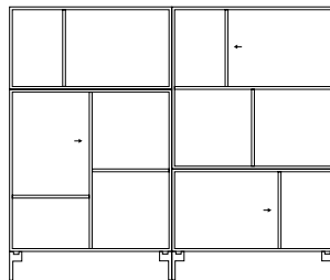
Shelving on legs with W 139.2 cm H 105 cm Legs 12.6 cm
