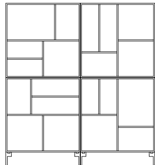
Shelving on legs W 139.2 cm H 139.2 cm Legs H 12.6 cm
