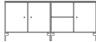
Lowboard on legs W 139.2 cm H 48 cm Legs 12.6 cm
