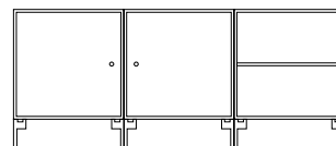
Shelving on legs W 140.4 cm H 46.8 cm Legs H 12.6 cm
