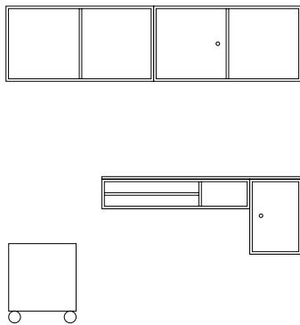
LINE D 30 cm W 139.2 cm H 35.4 cm BUREAU D 38 cm W 93.8 cm H 13.8/36.6 cm PLAY D 35.4 cm W 35.4 cm H 30 cm Castors H 6.8 cm
