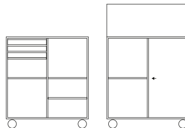
Mobile shelving x 2 D 30 cm W 69.6 cm H 69.6 cm Castors H 8 cm Living Things D 30 cm W 69.6 cm H 30 cm
