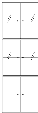
RISE D 30/46.8 cm W 69.6 cm H 208.8 cm Plinth H 3 cm
